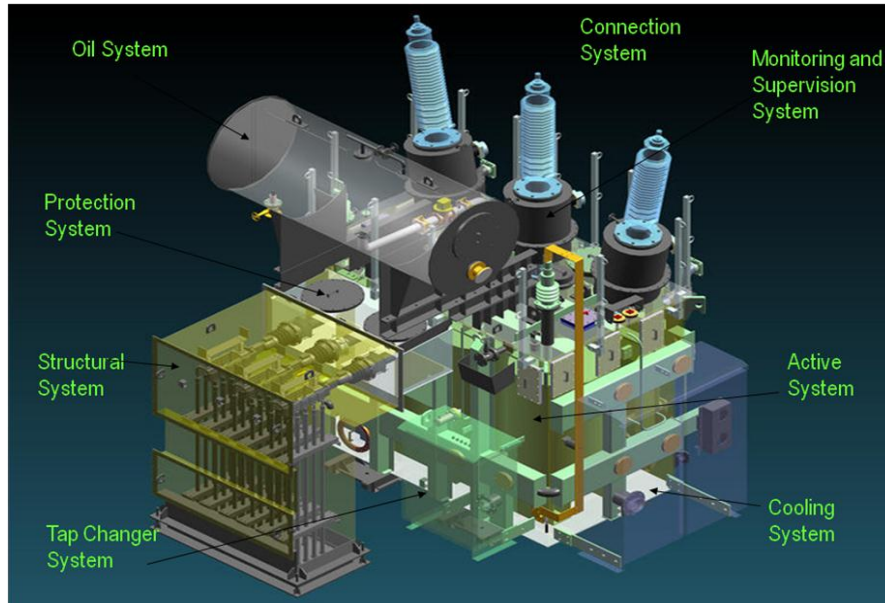
Figure 3 – Transformer Systems
