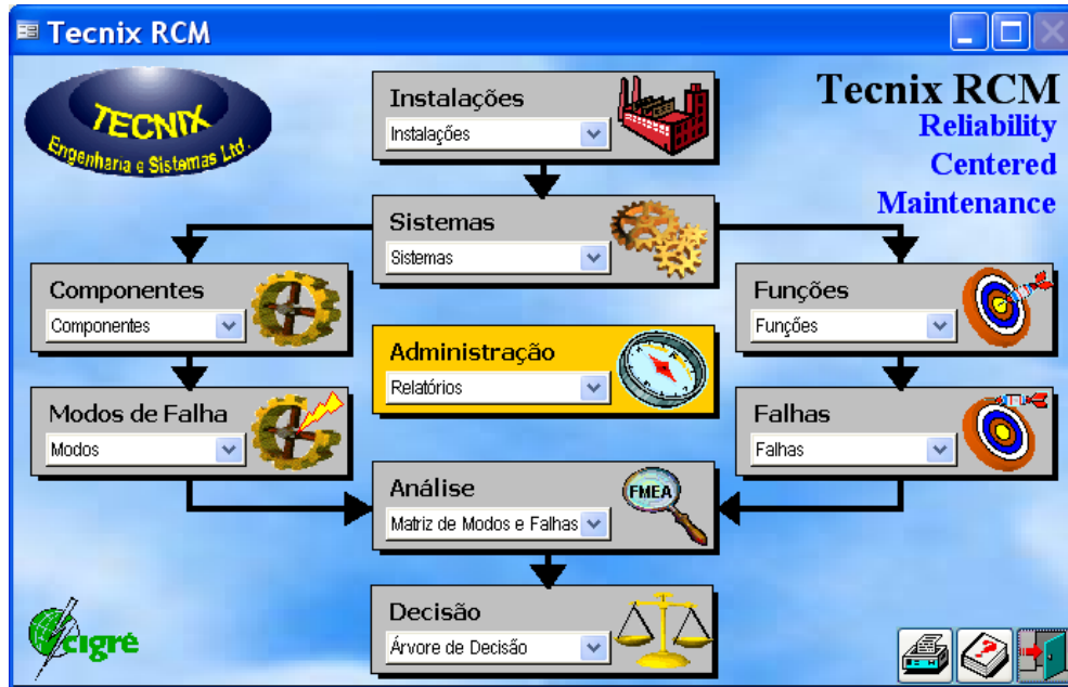
Figure 1 – RCM Software
