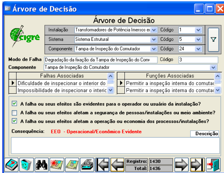
Figure 15 – Decision Tree Documentation
